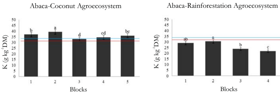
Fig. 3. Potassium concentration in abaca leaves planted in different blocks of the two agroecosystems showing the critical K concentrations in banana (blue line) and plantain (red line) leaves ( Note: Different letter superscripts (a-d) of same dependent variable among blocks are significantly different at p \leq 0.05 , n=40 in abaca-coconut and n=20 in Abaca-Rainforestation )
