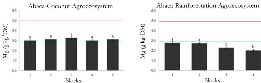
Fig. 5. Magnesium concentration in abaca leaves planted in different blocks of the two agroecosystems showing the critical Mg concentrations in banana (blue line) and plantain (red line) leaves (Note: Different letter superscripts (a-b) of same dependent variable among blocks are significantly different at p < 0.05 , n = 40 in abaca-coconut and n = 20 in Abaca-Rainforestation)
