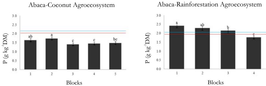
Fig. 2. Phosphorus concentration in abaca leaves planted in different blocks of the two agroecosystems showing the critical P concentrations in banana (blue line) and plantain (red line) leaves ( Note: Different letter superscripts (a-c) of same dependent variable among blocks are significantly different at p \leq 0.05 , n=40 in abaca-coconut and n=20 in Abaca-Rainforestation )
