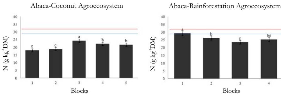
Fig. 1. Nitrogen concentration in abaca leaves planted in different blocks of the two agroecosystems showing the critical N concentrations in banana (blue line) and plantain (red line) leaves ( Note: Different letter superscripts (a-c) of same dependent variable among blocks are significantly different at p \leq 0.05 , n=40 in abaca-coconut and n=20 in Abaca-Rainforestation )
