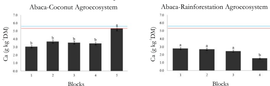
Fig. 4. Calcium concentration in abaca leaves planted in different blocks of the two agroecosystems showing the critical Ca concentrations in banana (blue line) and plantain (red line) leaves ( Note: Different letter superscripts (a-b) of same dependent variable among blocks are significantly different at p \leq 0.05 , n=40 in abaca-coconut and n=20 in Abaca-Rainforestation )
