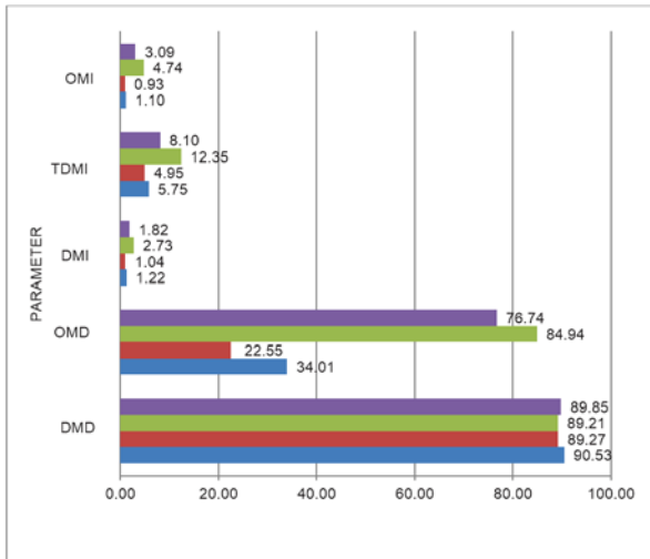
Figure 1. Average dry matter intake, dry matter digestibility, organic matter intake, total dry matter intake, and organic matter digestibility of goats fed with corn fodder based diets.
